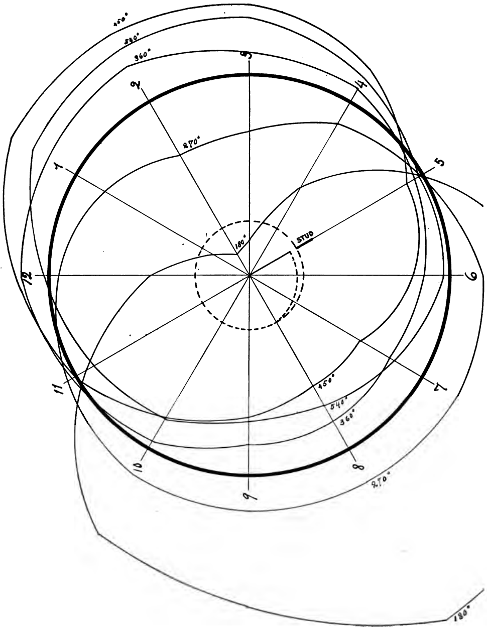
Plate VI.—Position Error of a Cylindrical Spring, Illustrating Table 7.
