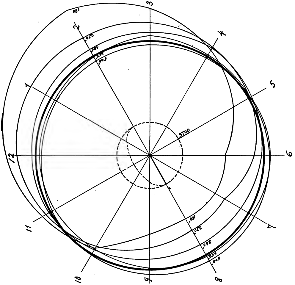
Plate X.—Position Error of a Cylindrical Spring with Theoretical Terminals, Illustrating Table 11.
