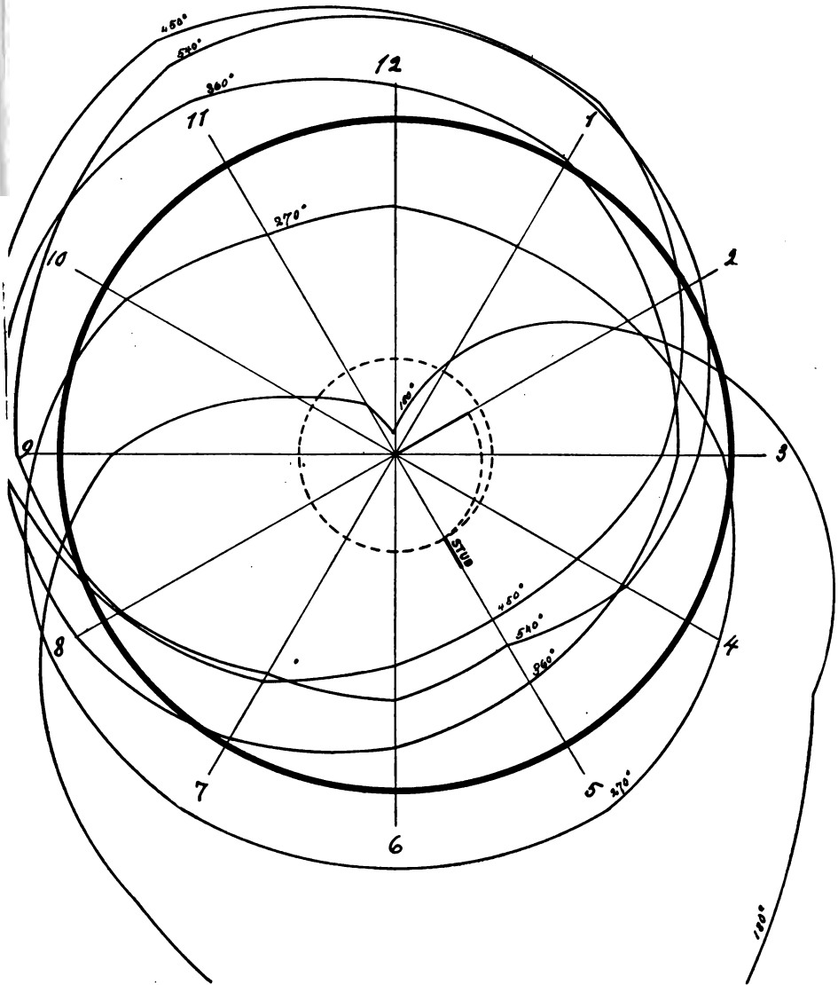
Plate VII.—Position Error of a Cylindrical Spring, Illustrating Table 8.
