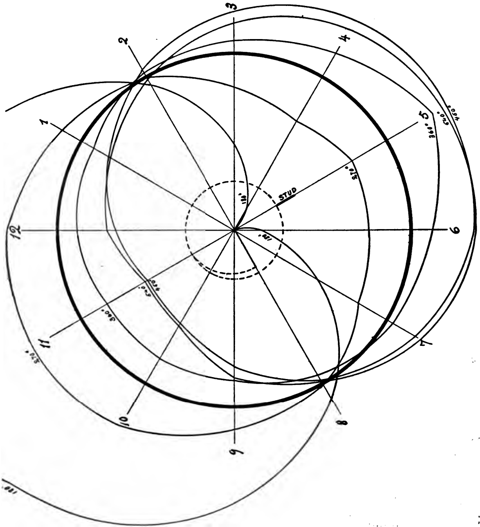
Plate IX.—Position Error of a Cylindrical Spring, Illustrating Table 10.
